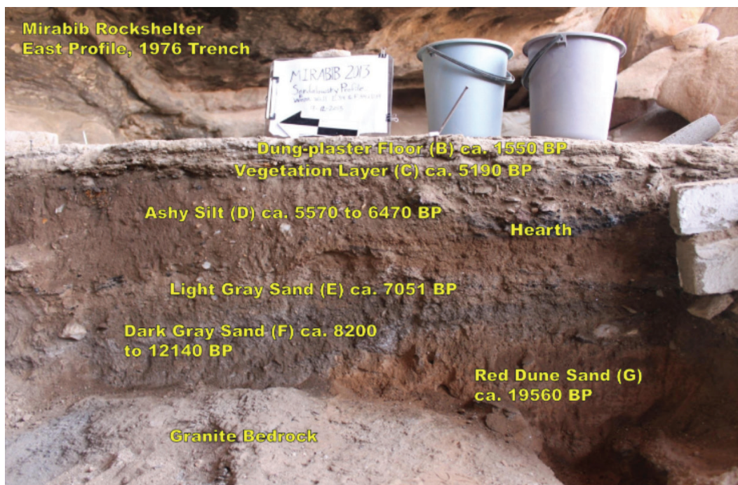
Figure 3: Profile of Sandelowsky's excavation trench reopened in 2013 showing the OSL and radiocarbon ages of the various layers at the site
