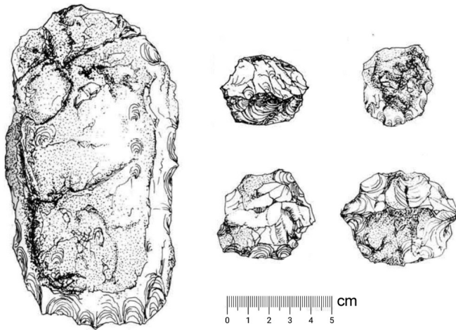
Figure 4: Typical lithics from the late Pleistocene lower levels at Mirabib. Left: scraper. Center/Right: scrapers/disoid cores. Drawings adapted after Sandelowsky (1977)
