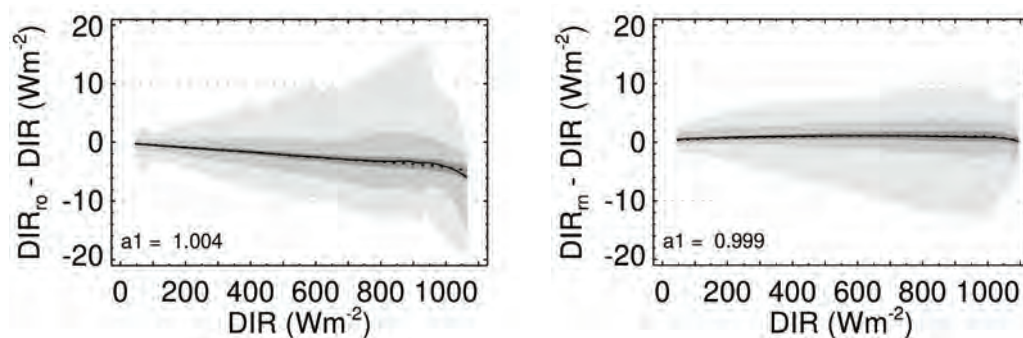
Figure 4: Differences in direct normal incidence between redundant measurements versus the BSRN instrument DIR, which operated continuously since June 2012. Left: for DIR 10 (redundant, old) from June 2012 to October 2013. Right: for DIR m (redundant, new) from November 2013 to March 2020. 1-min averages, class width is 30 W m -2 , average/median = solid/dotted line, grey areas contain 50, 90 and 99% of differences. a1 indicates the regression factor.
